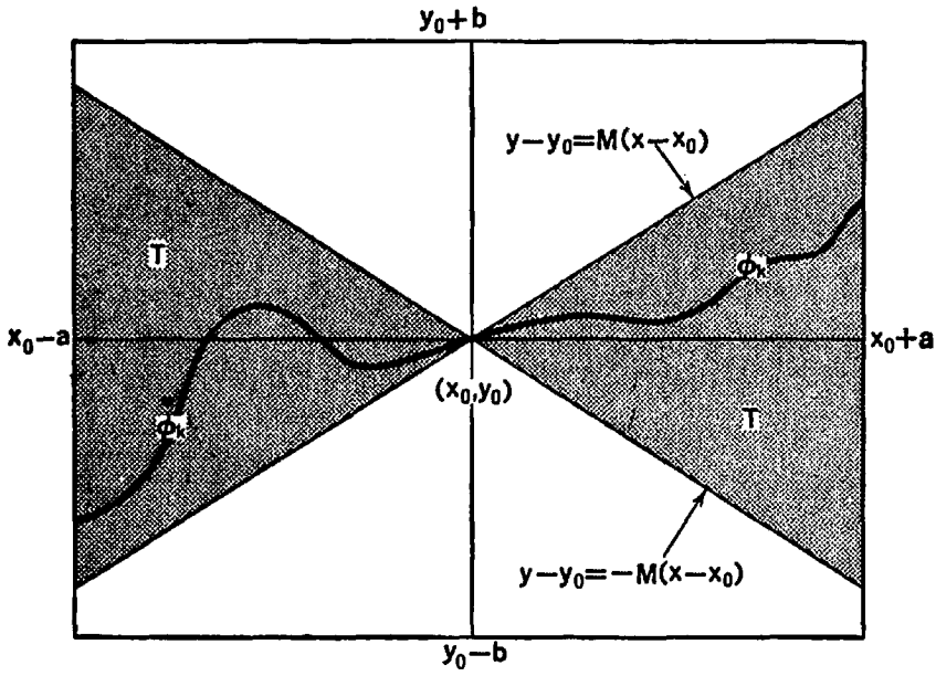
Figure 6. The region T(\alpha = a)
