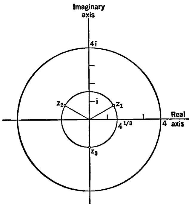
Figure 2. Three cube roots of 4i
