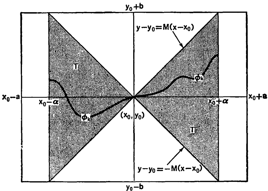
Figure 7. The region T(\alpha = b/M)
